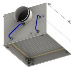
DISMANTLED HEPA FILTER PARTIAL ASSEMBLY
